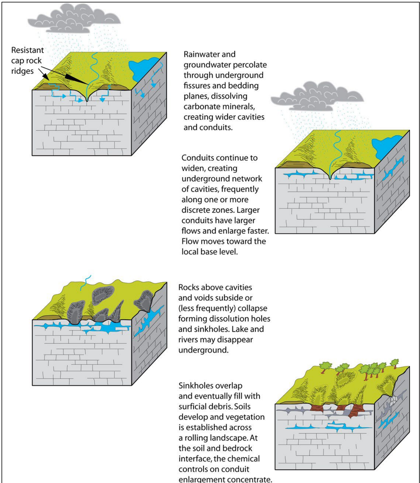
Figure 11-2. Formation of Sinkholes in Karst Terrain
